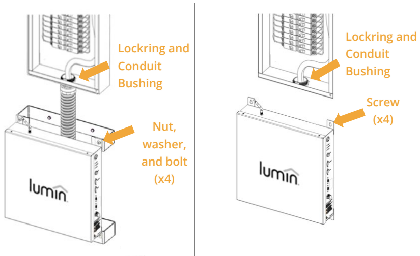
Surface-mounted installation
