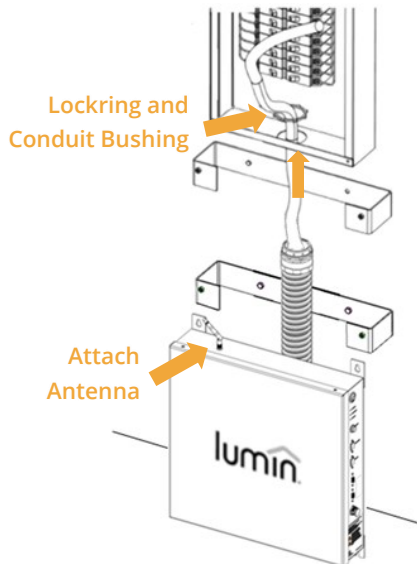
Surface-mounted installation
